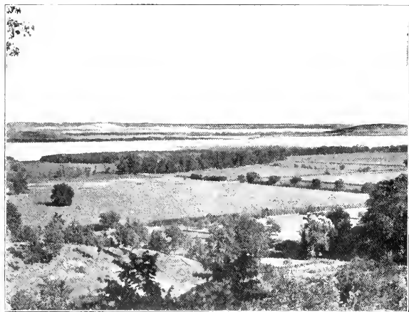
B. The flat in the middle foreground is part of an extensive terrace between Peoria and Mossville. The lower slopes of the valley side appear in the immediate foreground. (Photo by Dewein.)
